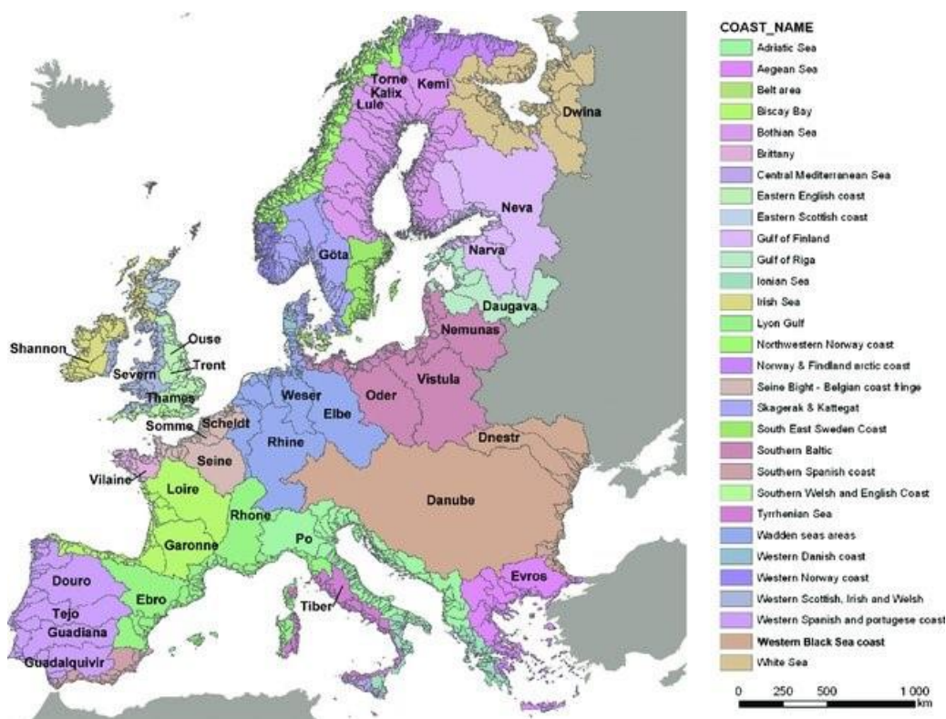
Figure 8. Major regional watersheds in Europe and their receiving coastal marine systems 19 .
